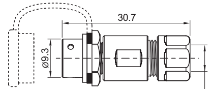
电缆直径: I: 3-4mm, II: 4-5mm (不标) Cable outer diameter range
