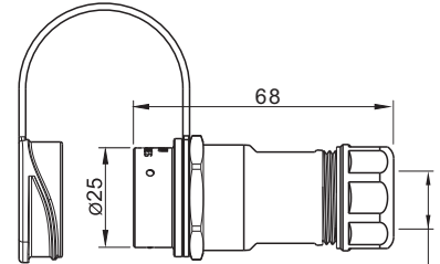
电缆直径: 10-14mm Cable outer diameter range
